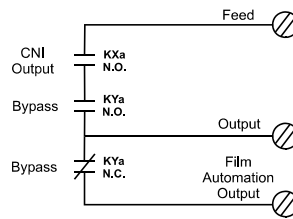
High Power Relay Contacts
